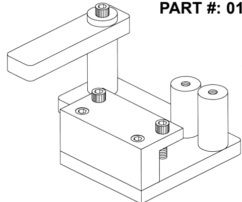
TROWEL ARM ALIGNMENT JIG
