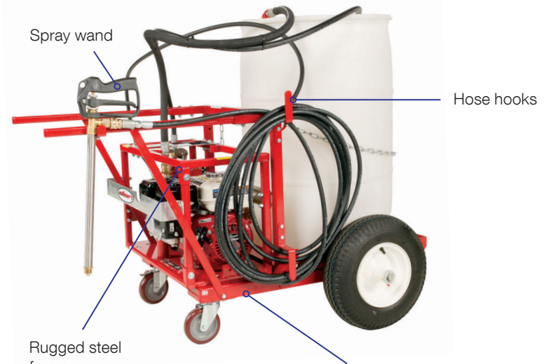
PS9910 shown with optional push cart (PSPCP-2)
